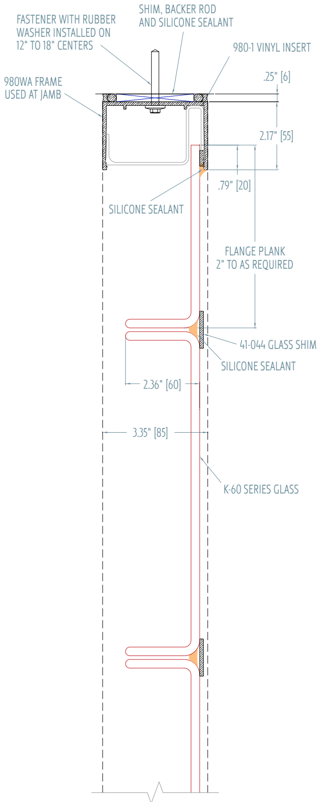
STANDARD SINGLE GLAZING
