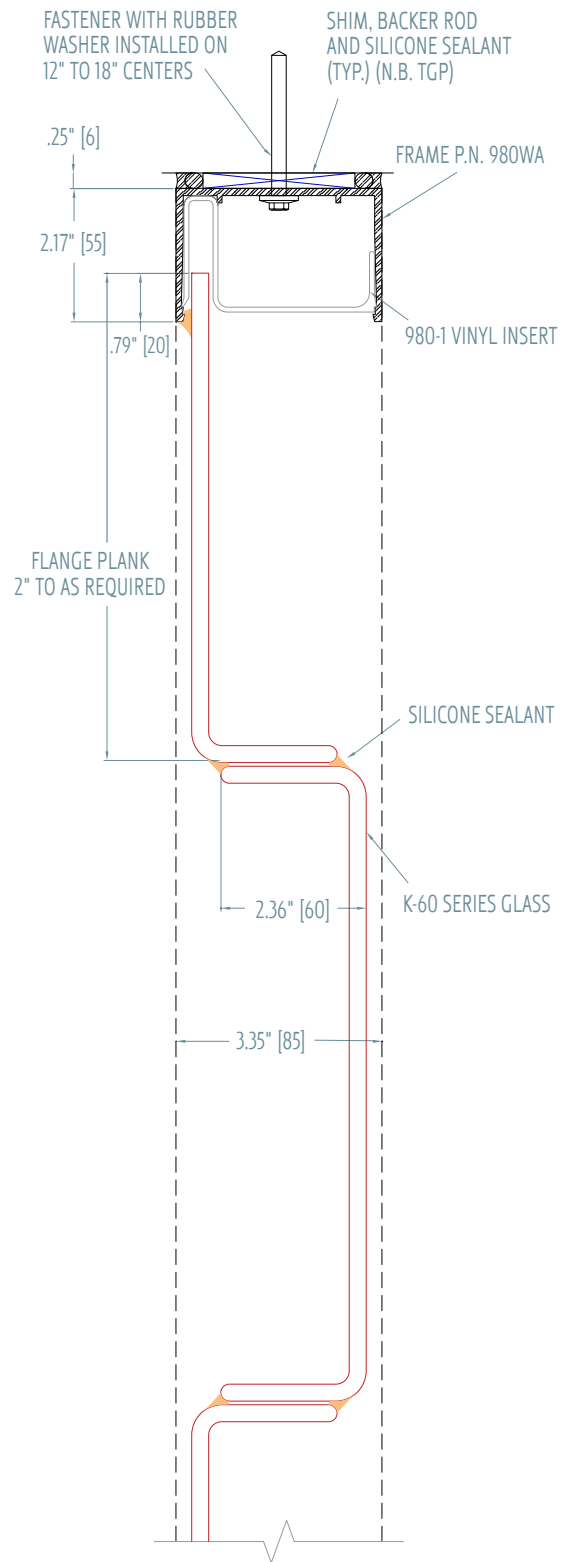
STAGGERED SINGLE GLAZING
