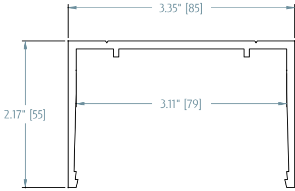
980WA HEAD / JAMB OR SILL FOR INTERIOR APPLICATIONS
