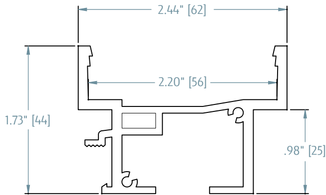
961WA SILL
